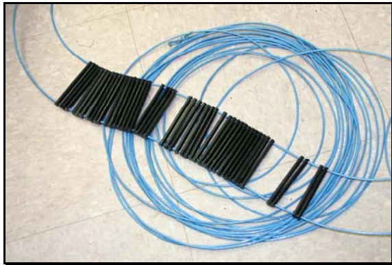
Figure 5 – Plastic spacers on the wire pair prior to being glued.
