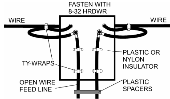
Figure 8 – Drawing of center insulator with additional strain relief for the antenna wire.
