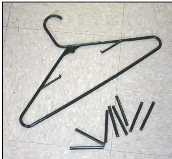
Figure 1 – Before and after spacer production made from cheap plastic coat hangers.
