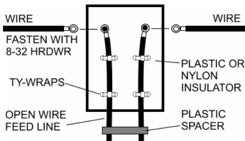
Figure 7 – Drawing of center insulator and balanced/open wire feed line.
