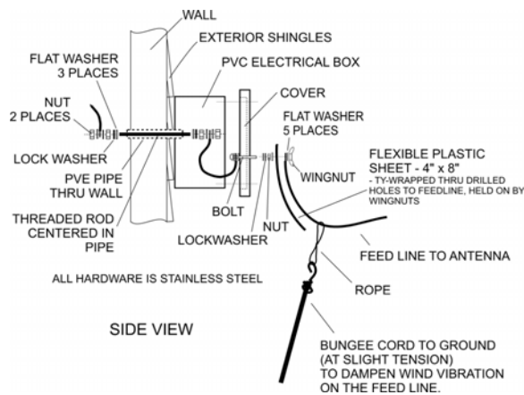
Figure 11 – Drawing showing detail of feeding balanced line through a building wall.
