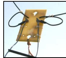
Figure 9 – Antenna end. The thing hanging from the bottom hole is a length of twine used to pull the antenna down to working level.
